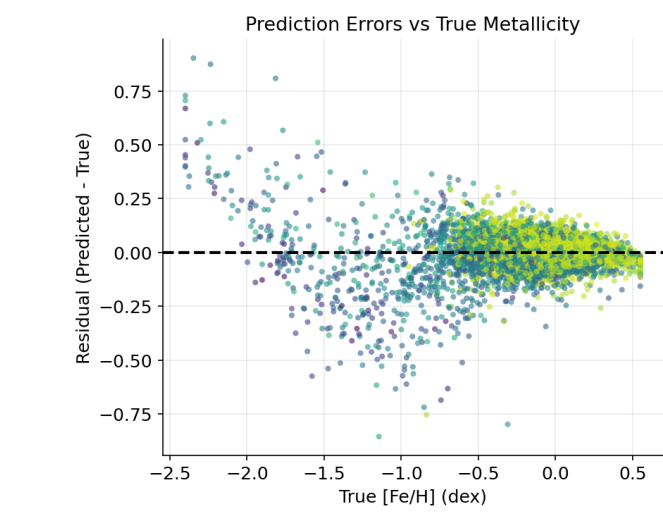
Figure 6. Residuals and Uncertainty
