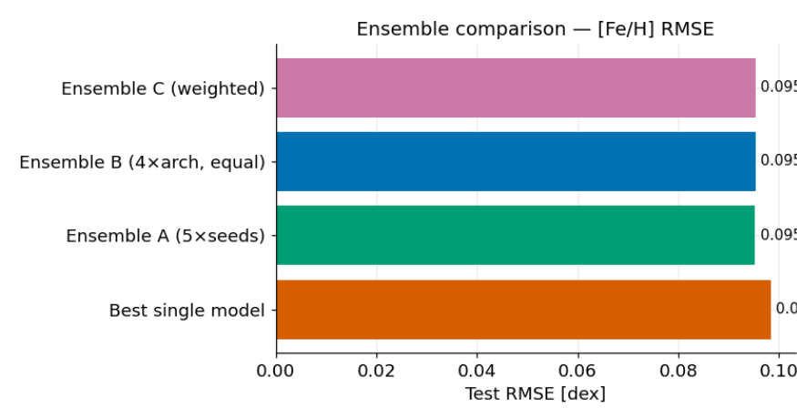
Figure 1. Test RMSE Comparison of Neural Network Ensembles
