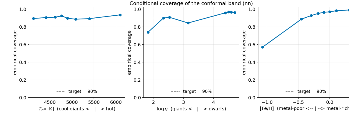
Figure 3. Coverage Varies Across Stellar Parameter Space
