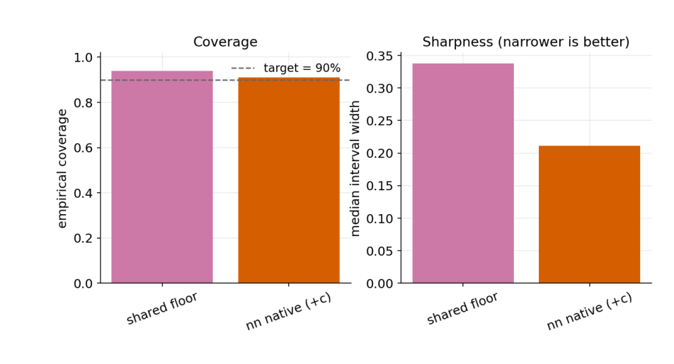
Figure 7. Coverage and Sharpness
